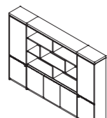
文件柜 EF98 Cabinet W2796*D396*H2000
