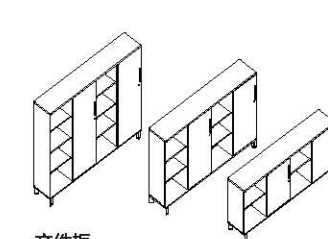
文件柜 DE96 2352(W)*437(D)*880(H) 2352(W)*437(D)*1278(H) 2352(W)*437(D)*1584(H)
