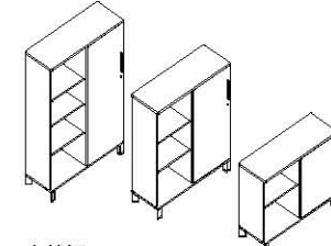
文件柜 DE92 1188(W)*437(D)*880(H) 1188(W)*437(D)*1278(H) 1188(W)*437(D)*1584(H)
